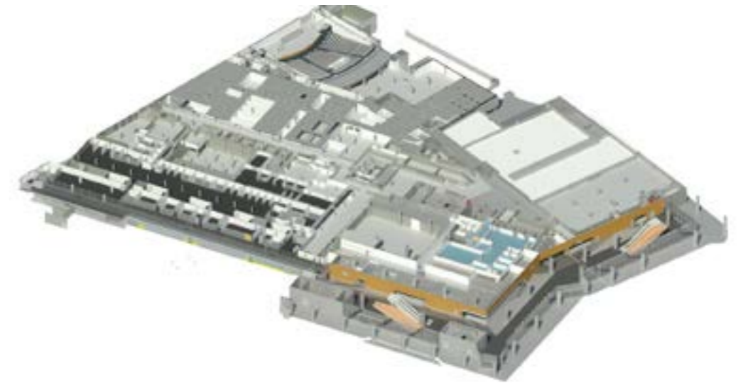
Axonometric cutaway view of Level 1 Convention Centre
