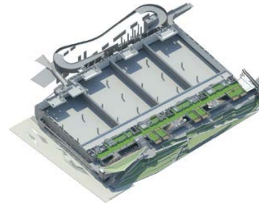
Axonometric cutaway view of Level 3 Exhibition Centre
